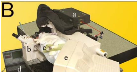
Figure 3. Corneal multiphoton microscopy with living animals. (A). As illustrated on the schematic drawing, the ultrashort laser pulses were deflected into the multiphoton microscope and then conveyed into samples through a scanning unit built up in the microscopical system. The emitted lights including autofluorescence and second harmonic generated signals were separated from the incident lights by a filter cube and then guided into PMT in a backward direction; (B). On-site photograph for overview of multiphoton imaging system. The animal was being imaged under the inverse multiphoton microscope. The optical mirrors deflecting the laser beams are illustrated in a simplified way on this photograph. a) compact mode-locked tunable 90 MHz Ti:sapphire laser Chameleon; b) multiphoton microscope based on the inverse Zeiss LSM; c) animal during imaging; d) wavelength tuner; e) imaging monitor; (C). Frontal photograph showing a rabbit being imaged under the multiphoton microscope. The animal was narcotized by intravenous narcotics ketamine and xylazine. The blood oxygen concentration and pulse frequency of the being treated animal was totally monitored from begin to end during the non-linear optical imaging by a Dräger Dialogue 2000. Insert (D). Image taken from underside of the sample stage showing the animal eye being treated.
